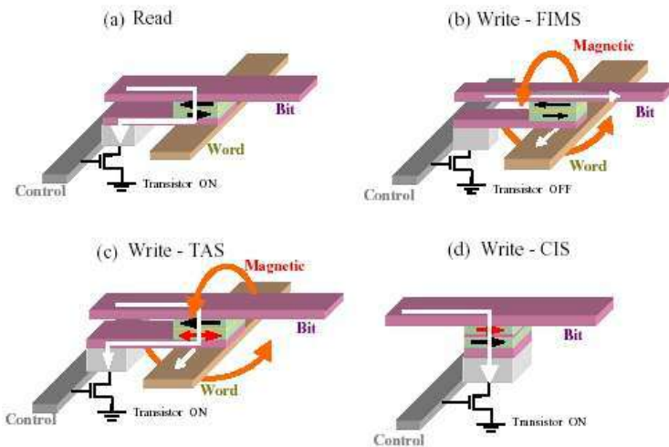
Figure 2: Read and write principles of MRAM with various architectures: (a) Read (common principle); (b) Write in FIMS (Field Induced Switching) mode; (c) Write in Thermally Assisted Switching (TAS) mode; (d) Write in Current Induced Switching (CIS) mode
